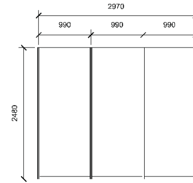
ELEVATION(back wall)
